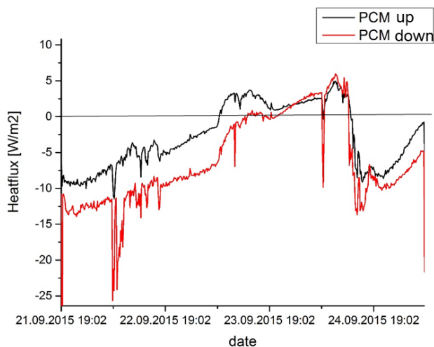
Figure 8: Heat Flux through PCM window (top and bottom) when there is no sun for several consecutive day
